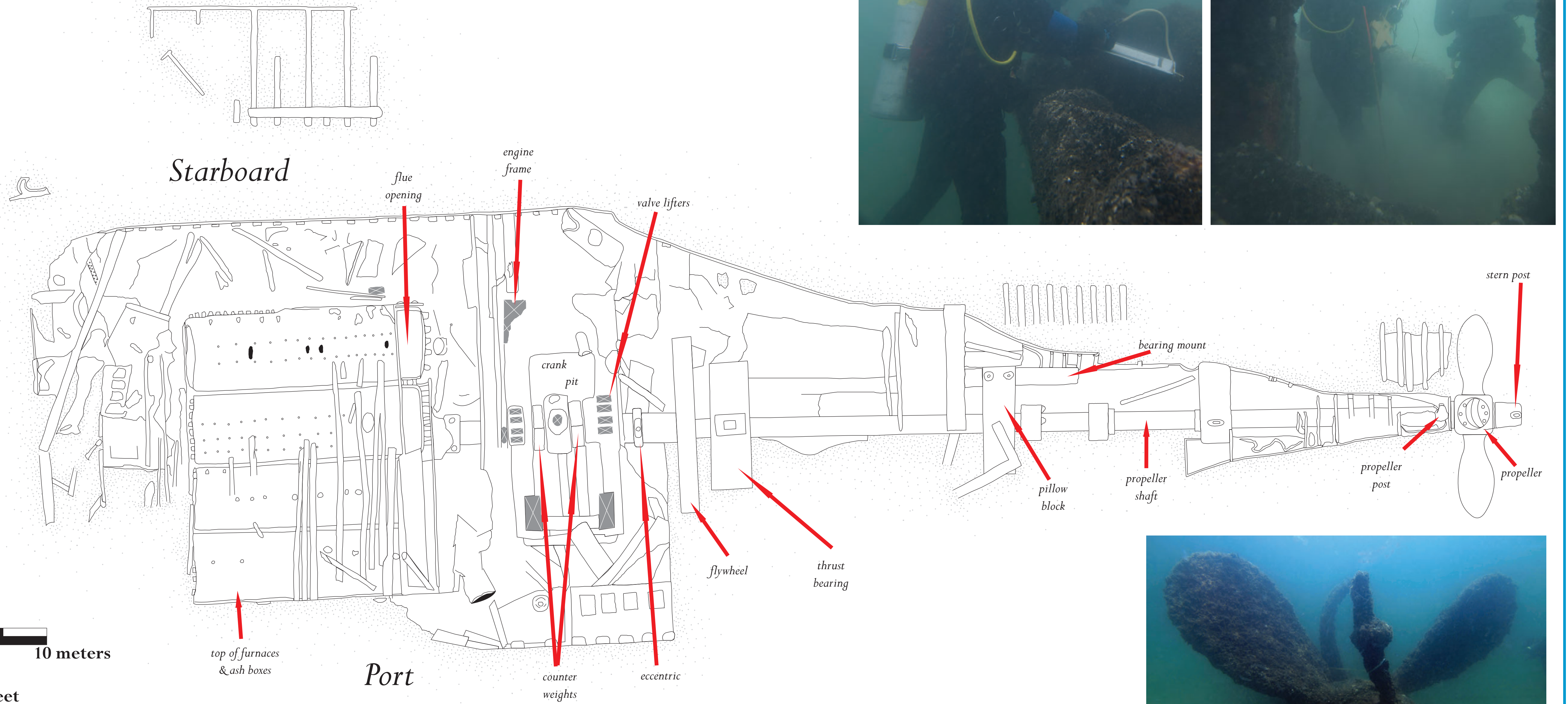
Propeller blades (view towards bow) Photo: John McCord/UNC-CSI
